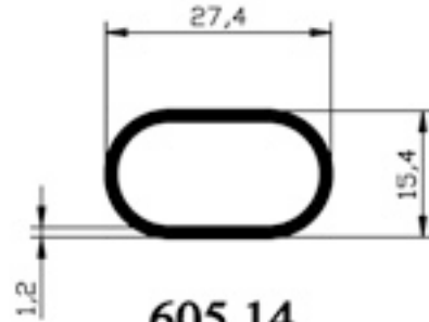
605.14 OVAL BORU 0.220 gr/m
