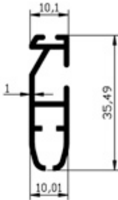
108.12 STOR ALT PARÇA 0.251gt/m
