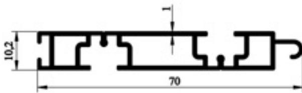
107.06 PANJUR KİLİT PROFİLİ 0,533gr/m
