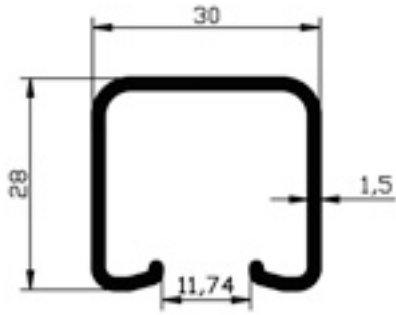
201.18 0.380gr/m RAY
