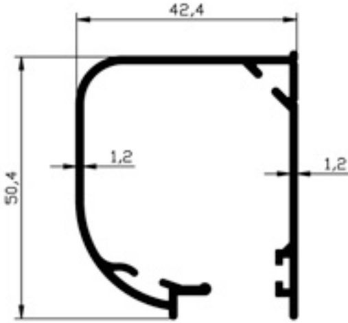
108.10 STOR KASA 0.598gt/m
